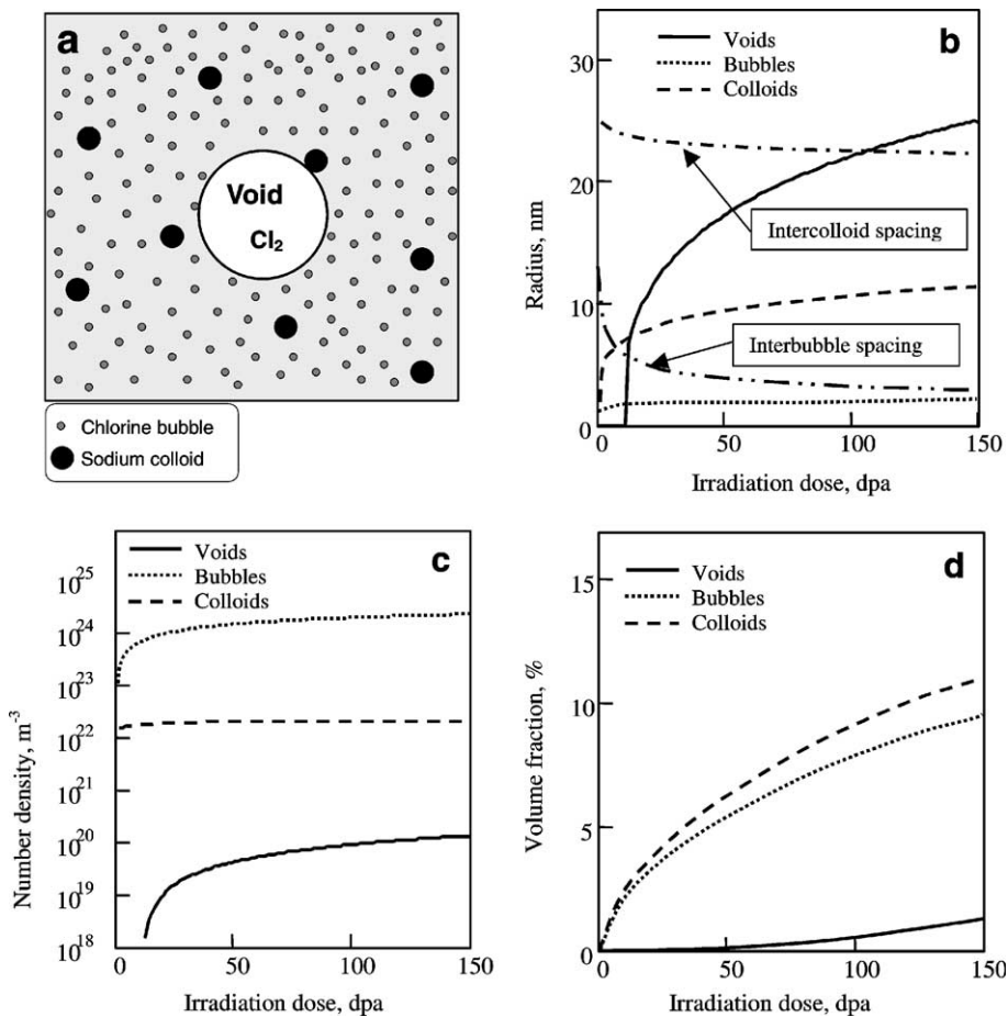
Fig. 2. Evolution of bubbles, colloids and voids with increasing irradiation dose (in displacements per anion, dpa) calculated for the laboratory irradiation conditions ( 100\text{ }^\circ\text{C} , 3 \times 10^{-5} dpa/s) and a constant dislocation density 10^{14}\text{ m}^{-2} [14]. (a) Graphic illustration; (b) Intersection between the colloid radius and interbubble spacing curves indicates a beginning of the explosive back reaction due to collisions between the bubbles and colloids resulting in the formation of voids, which grow to sizes exceeding the intercolloid spacing and thus provide for the following and larger step of the explosive back reaction; (c) and (d) show the corresponding number densities and volume fractions of radiolytic products.
